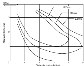
MMU-UP0481HP-E, UP0561HP-E
