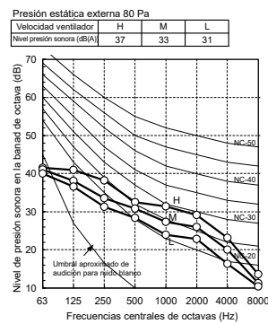
MMD-UP0481BHP-E, MMD-UP0561BHP-E
