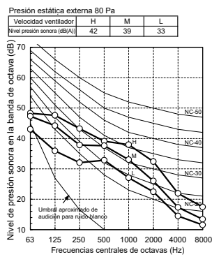
MMD-UP0301BHP-E
