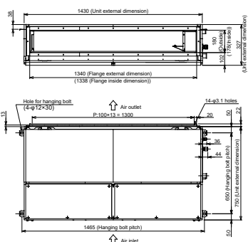
MMD-UP0481HFP-E
