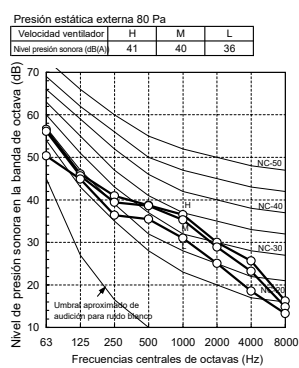
MMD-UP0481BHP-E, MMD-UP0561BHP-E
