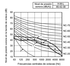
MMU-UP0561WH-E
