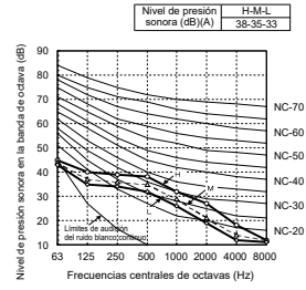
MMU-UP0241WH-E, UP0271WH-E
