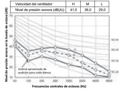
MMC-UP0561HP-E
